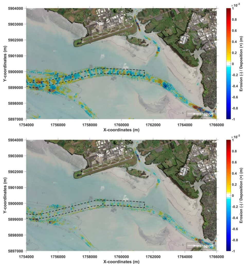
Figure B-6 Maps of erosion (negative, blue) and deposition (positive, red) results (Control 3) for runs using 150\ \mu m fraction (top) and 500\ \mu m (bottom). Note the difference in scale for the erosion/deposition in the inner harbour maps.
