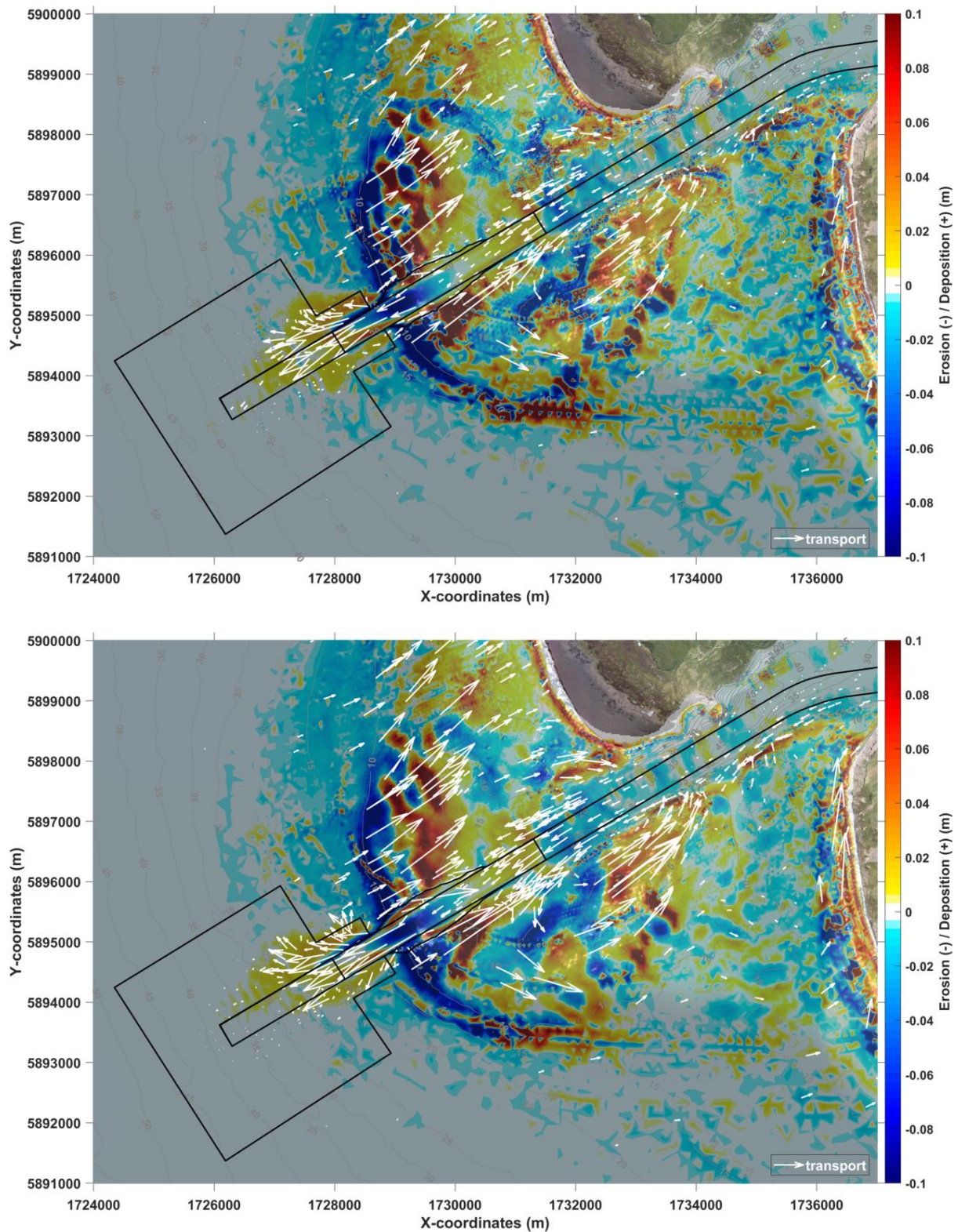
Figure 5-15 Maps of erosion (negative, blue) and deposition (positive, red) results for runs including the channel and forced by southwest waves ( H_s = 5 m, T_p = 15 s and Dir = 230 deg). Top map shows results for Control 7 runs using the original bathymetry and bottom map is for Control 7 with modified initial bathymetry represented by a post-storm condition and with accumulation dredged to design depth.
