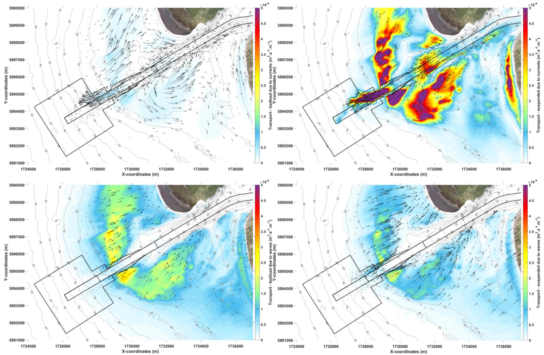
Figure 4-26 Maps of average bedload (left) and suspended (right) sediment transport for runs including the channel (Control 7, H_s = 5 m, T_p = 15 s and \text{Dir} = 230 deg). Top row shows transport due to currents and bottom row shows transport due to waves.
