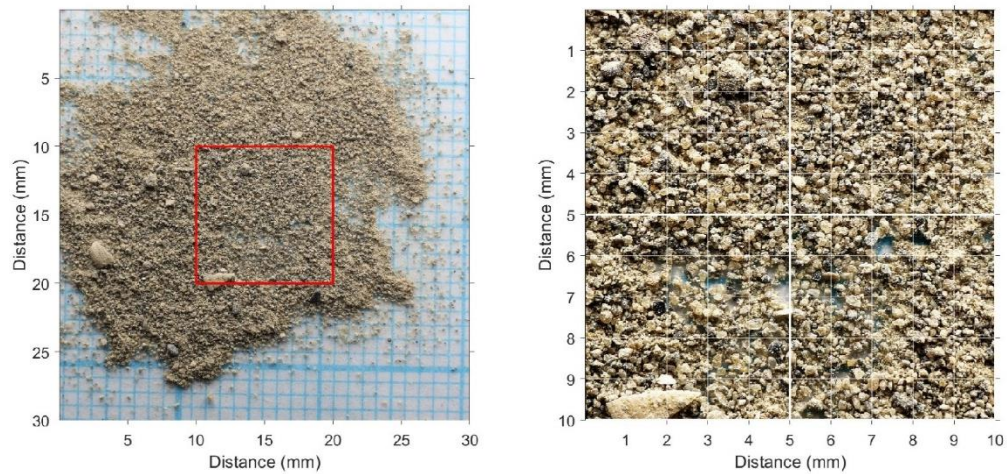
Figure 2-2: Sediment samples showing grain characteristics.
