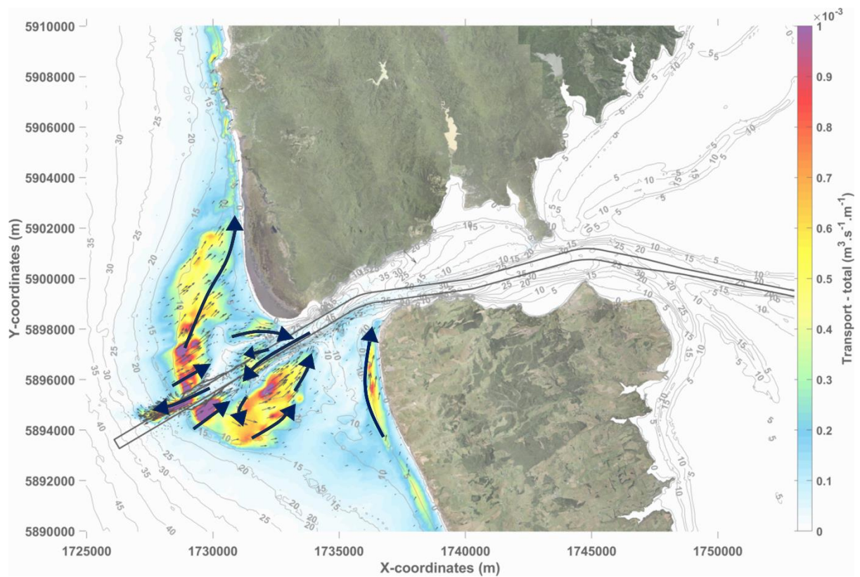
Figure 4-33 Sediment transport magnitude (colormap) and direction (thin black arrows) for runs including waves ( H_s = 5 m, T_p = 15 s and Dir = 230 deg). Control 3, existing bathymetry (top) and Control 7, bathymetry including the concept navigation channel (bottom). Bold blue arrows represent the main transport pattern.
