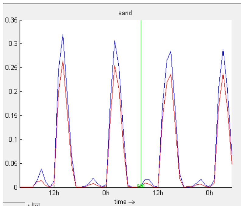
Figure 3-12 Sediment concentration ( \text{kg/m}^3 ) for two sites next to each other (red and blue lines) near the approximate location of field deployment. Green line represents the time of field sampling.
